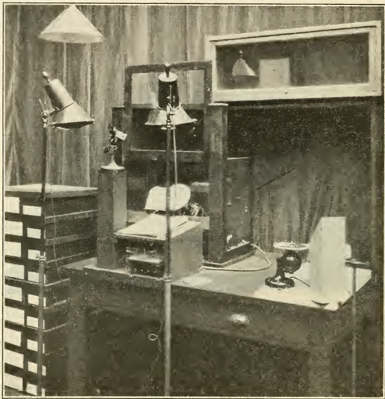
FIGURE 9.—First set-up for measuring the color of cotton using a comparator eyepiece. Note that the cotton is in juxtaposition to the color disks and that the lights are so placed as to give a definite angle on the disk surface. This set-up, modified as to the container for the sample, could be used for any other product that presents an even or a nearly even surface for measurement. The equipment has already been used for measuring the color of bread, cheese, condensed milk, and cotton cloth.
